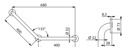
Installation example for WCs
