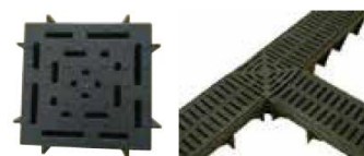
Square Hub-PL3004
